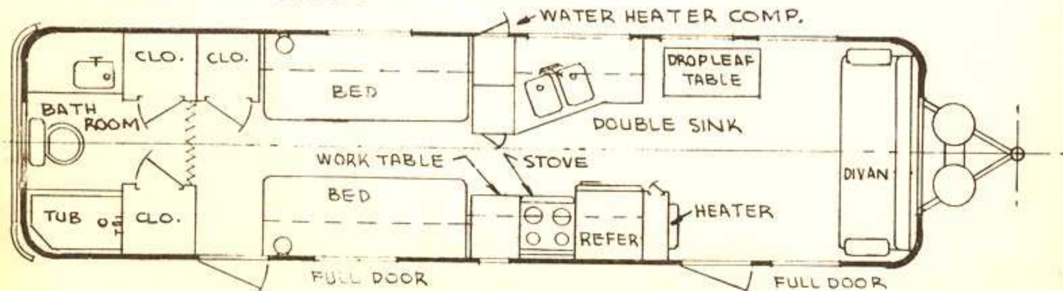
31' LUXURY LINER
