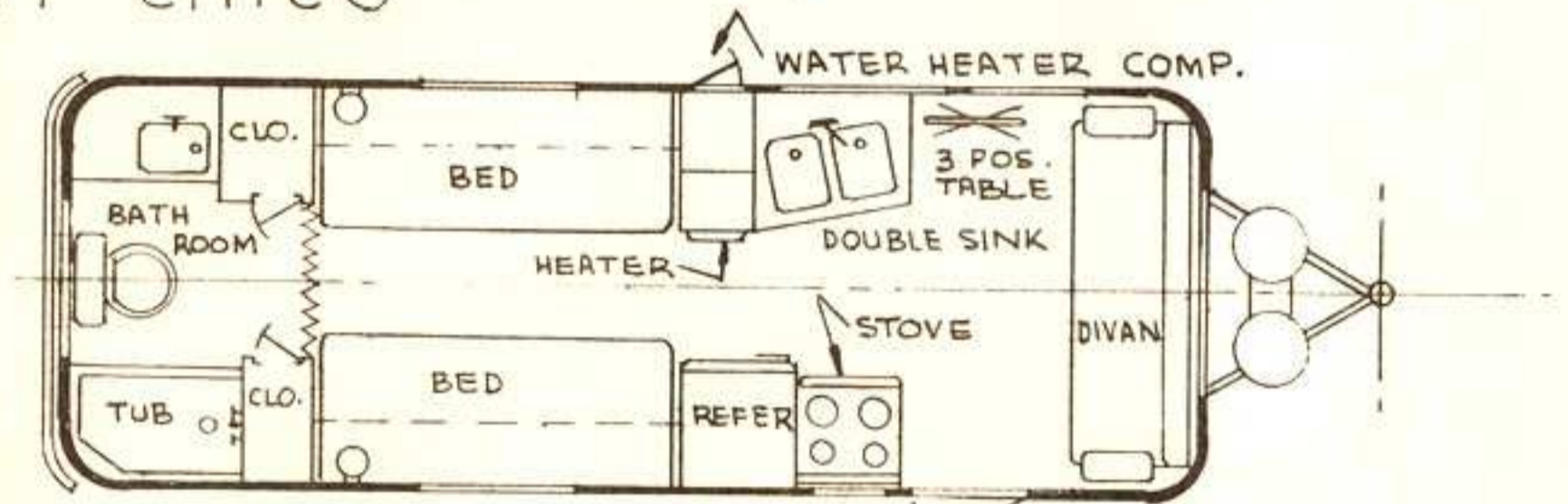
23' CLIPPER
